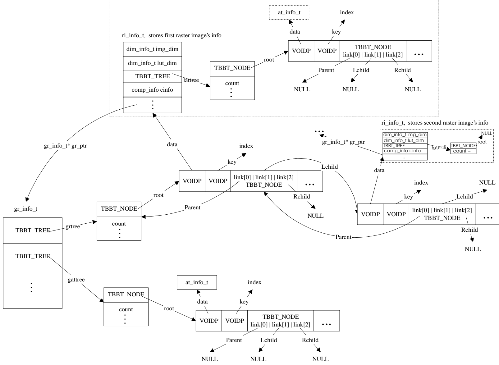
Data structures after adding two attributes
