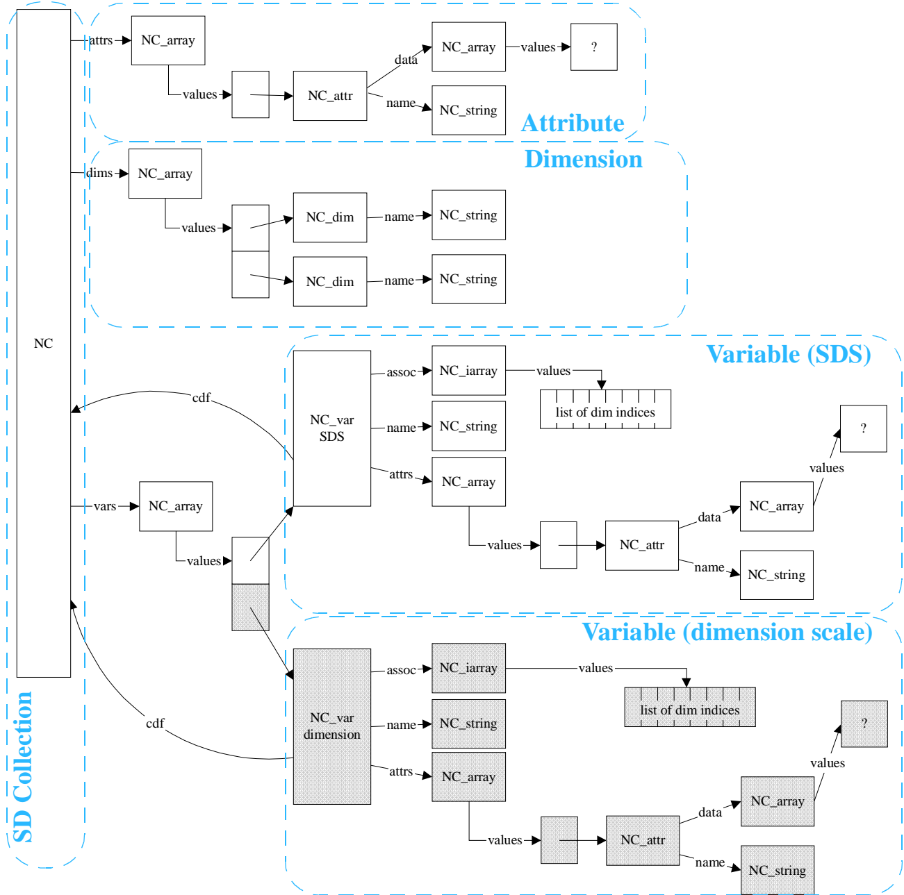
FIGURE 7y Example of HDF memory structures describing an SD collection
