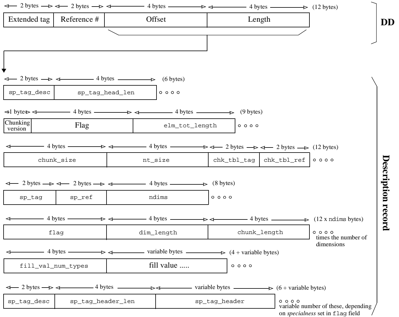
FIGURE 10g DD for a chunked element (12 bytes) pointing to a chunked element description record (>52 bytes)
