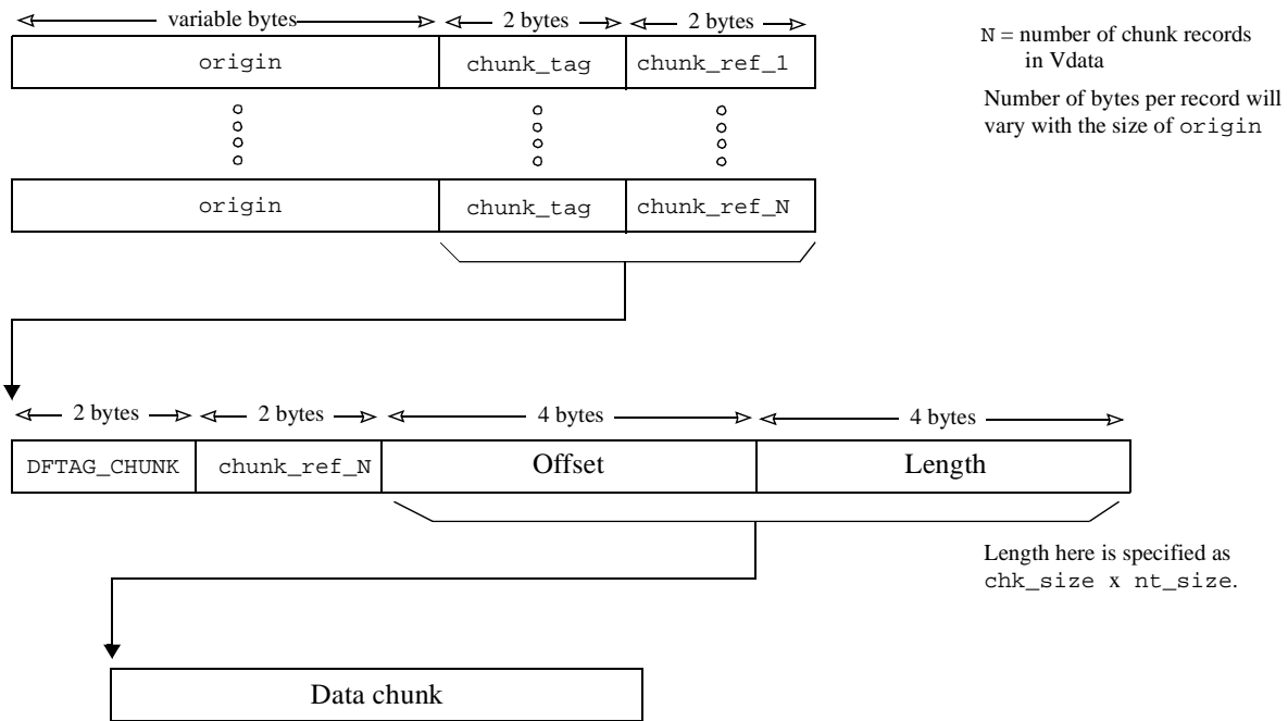
FIGURE 10h Chunk table
