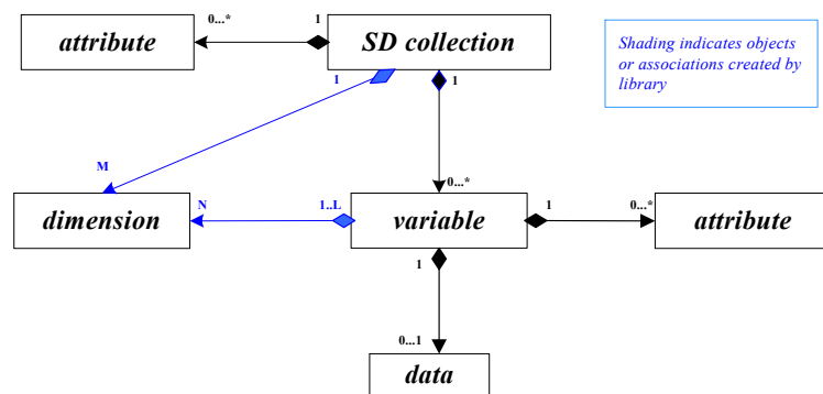
SD Developer's Model -- The SD Model from the Developer's Point of View
