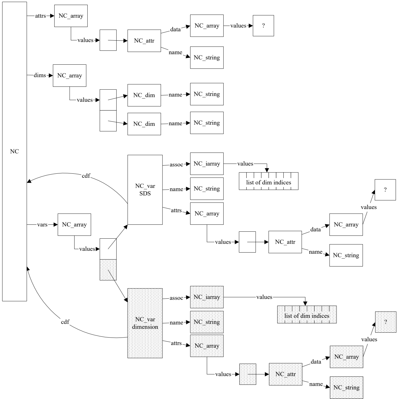
FIGURE 7y SD collection contents in memory after adding a dimension attribute
